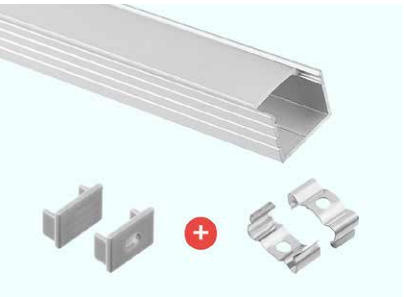
Aluminium frame set 3 (Art. BAC-ALU3-SET)
